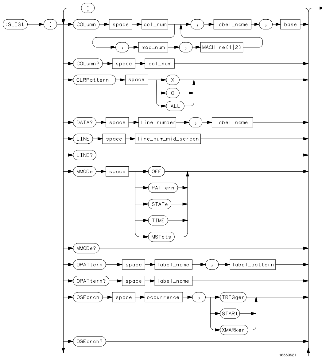
SLISL Subsystem Syntax Diagram
